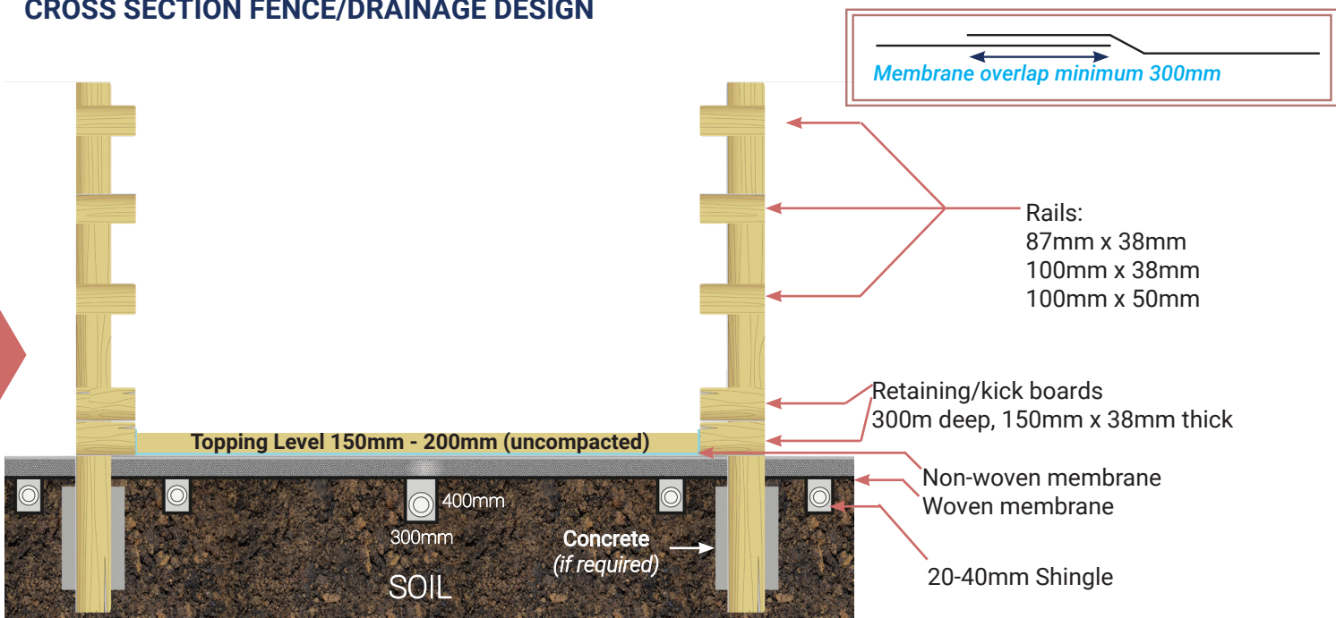
Standard 2.1m posts (longer 2.4m post option) Standard post section supplied 125mm x 75mm, also stocked 150mm x 75mm
