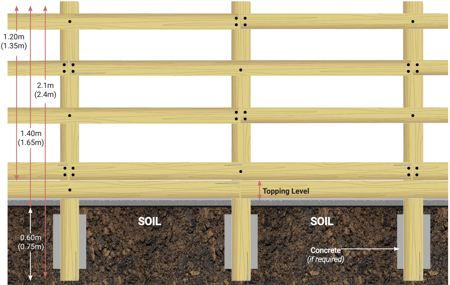
Standard 2.1m posts (longer 2.4m post option) Standard post section supplied 125mm x 75mm, also stocked 150mm x 75mm
