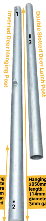
3 Double slotted latch posts, with a long oval shape slot, allowing for any drop in gate
