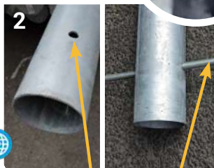
2 A pre-drilled 16mm hole at foot of post to add re-bar strength (re-bar can be supplied as extra)
